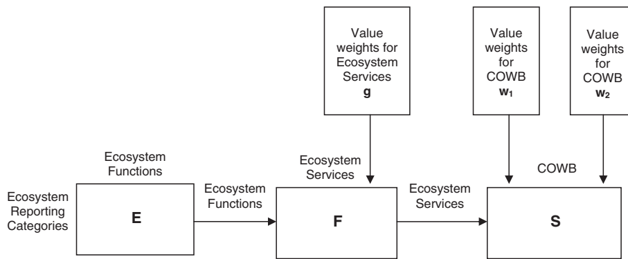
Fig. 1. The conceptual framework underpinning the scoring system in the SEQ ecosystem services framework.
